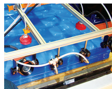
Model 8192 Gen4 Ion Air Cannons provide static elimination in between solar panel lenses to assist separation of the lenses during production.
