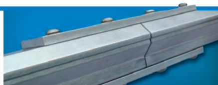
The Model 110900 Coupling Bracket Kit is used to join two aluminum Super Air Knives.
